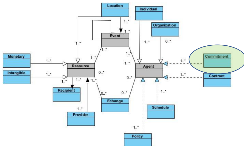
Fig. 57. REA Model. Source: Author’s own creation based on [19] and [324].
