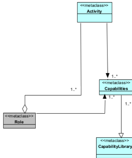
Fig. 21 Capability and CapabilityLibrary Metaclasses in M1/2 Cognitive Level of DIH Model Representation.
